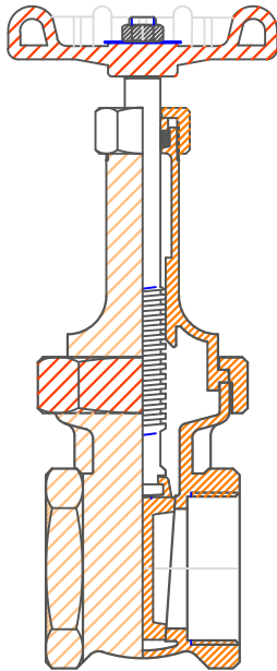
Fig. SW-205U for union bonnet
